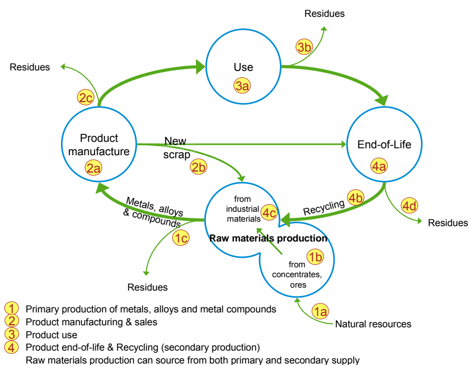
Figure 14: Life cycle of products/metals with principal points of intervention to improve resource efficiency. Source: modified after C.E.M. Meskers, Coated Magnesium – designed for sustainability? Dissertation Delft, 2008.
